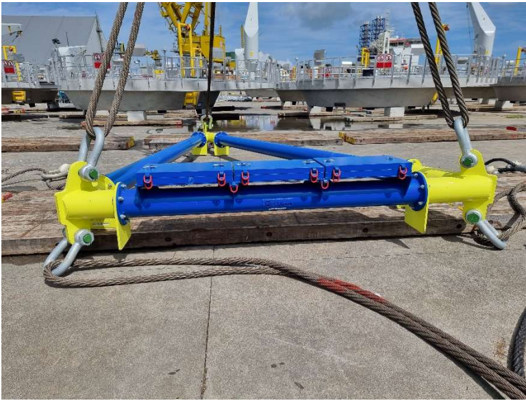
Figure 1, CWP loadspreader with rigging attached
